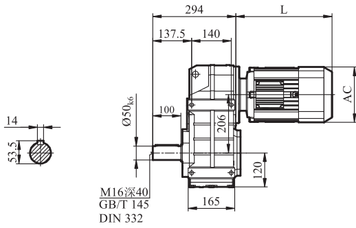
GFA/GFH/GFV77
