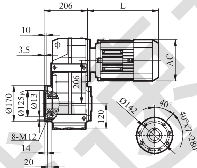
GFAF/GFHF/GFVF77
